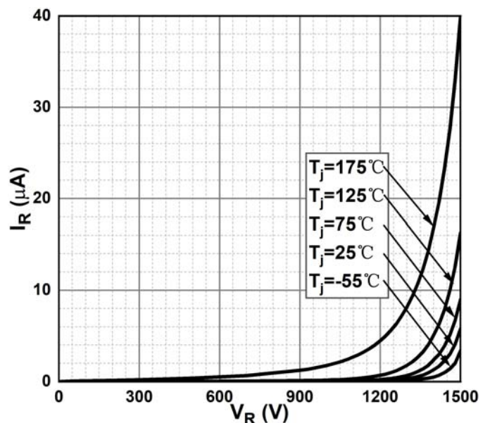
Figure 2. Reverse Characteristic
