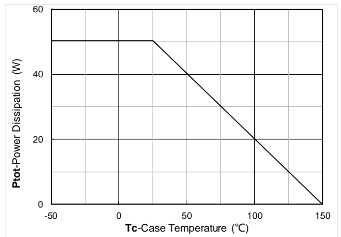
Figure 12. Power dissipation
